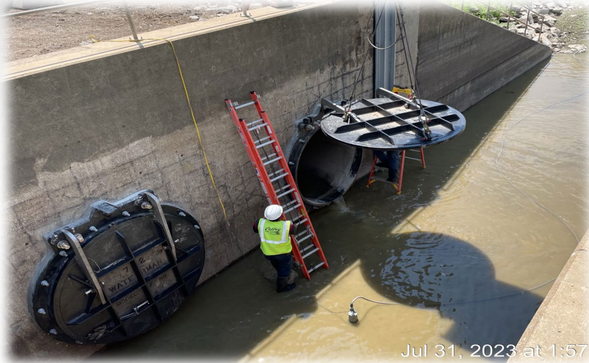
FRITZ FLAP GATE
